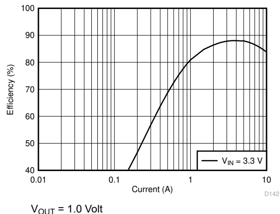
图 8-2. Efficiency in Forced-PWM-Four-Phase mode
