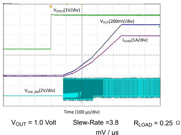
图 8-7. Start-Up With EN1, Forced-PWM-Four-Phase Mode
