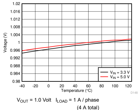
图 8-5. Output Voltage vs Temperature
