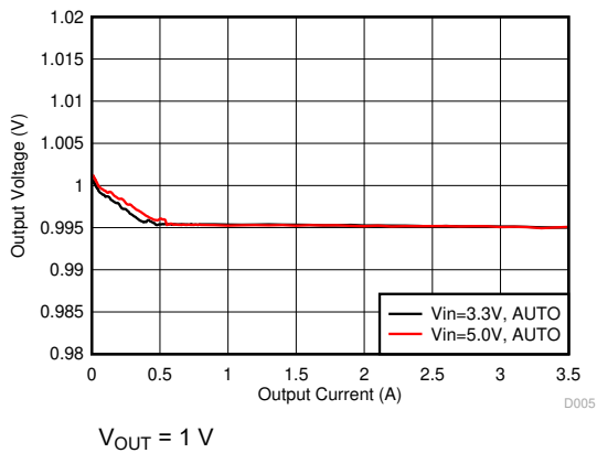
图 9-7. Buck Output Voltage vs Load Current in AUTO Mode
