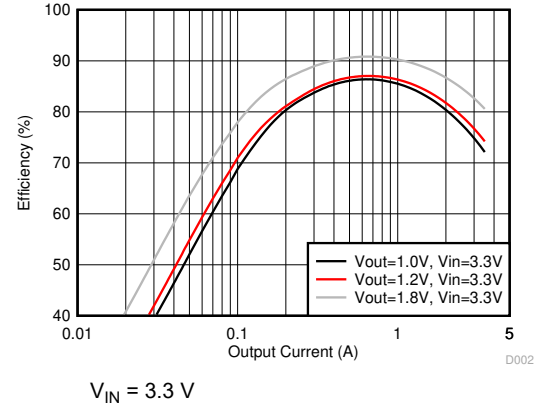
图 9-4. Buck Efficiency in Forced PWM Mode
