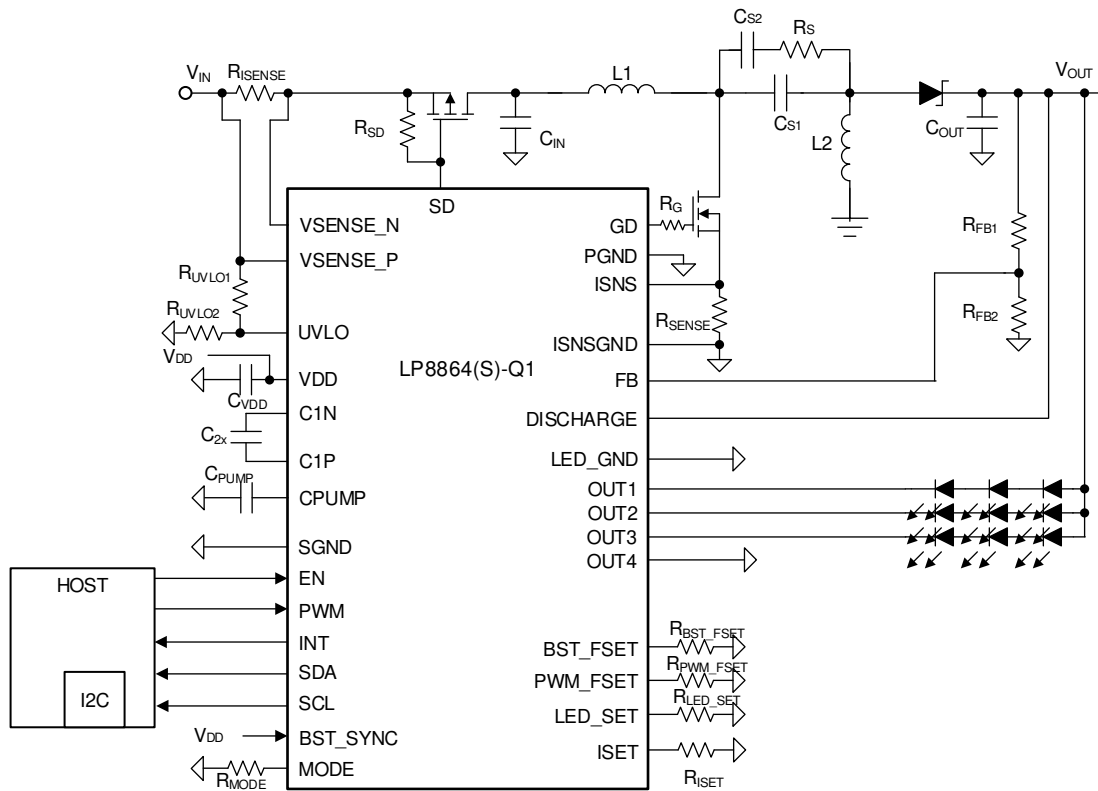
图 7-6. SEPIC Mode with Three LEDs in Series
