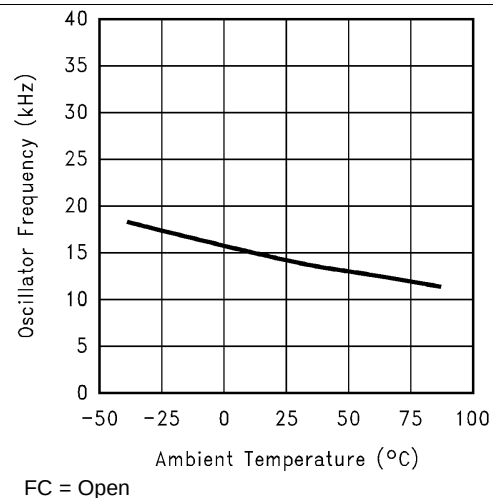
Figure 12. Oscillator Frequency vs Temperature
