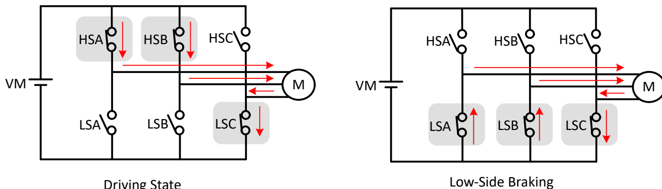
图 7-43. Low-Side Braking
