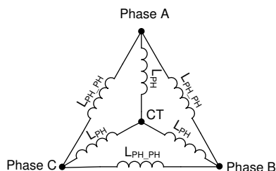
图 7-35. Motor Inductance
