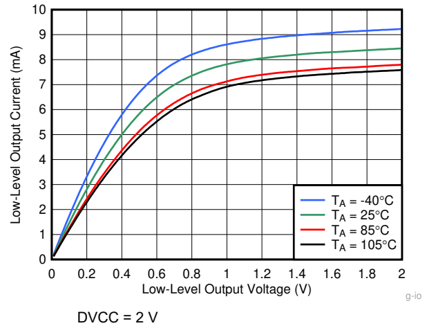
图 8-8. Typical Low-Level Output Current vs Low-Level Output Voltage
