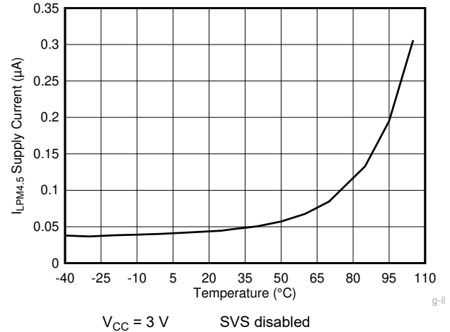
图 8-4. LPM4.5 Supply Current vs Temperature
