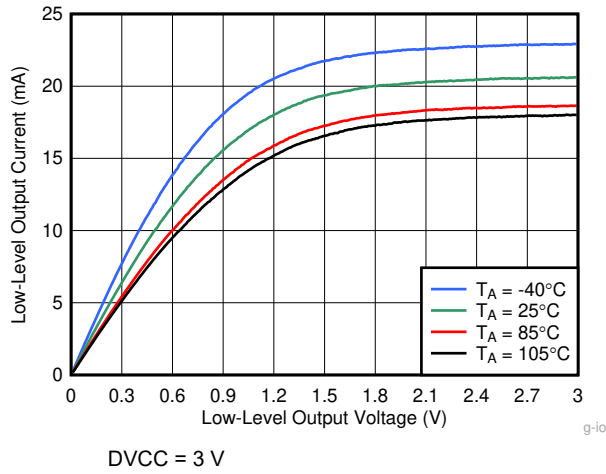
图 8-7. Typical Low-Level Output Current vs Low-Level Output Voltage
