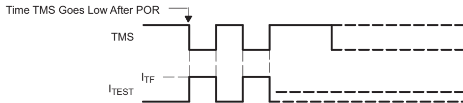
Figure 25. Fuse Check Mode Current
