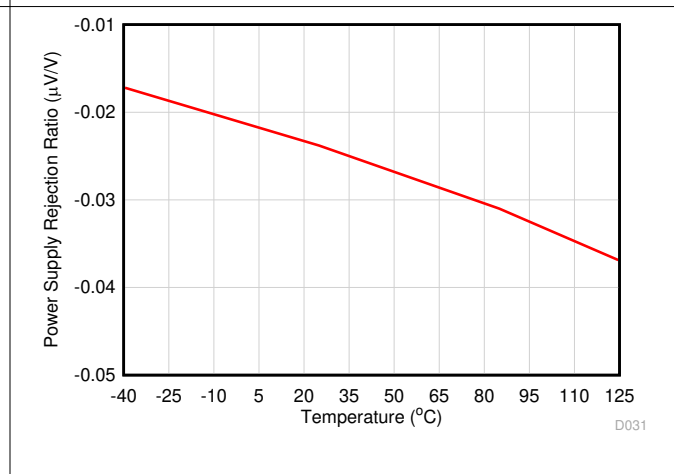
图 6-10. Power Supply Rejection Ratio vs Temperature
