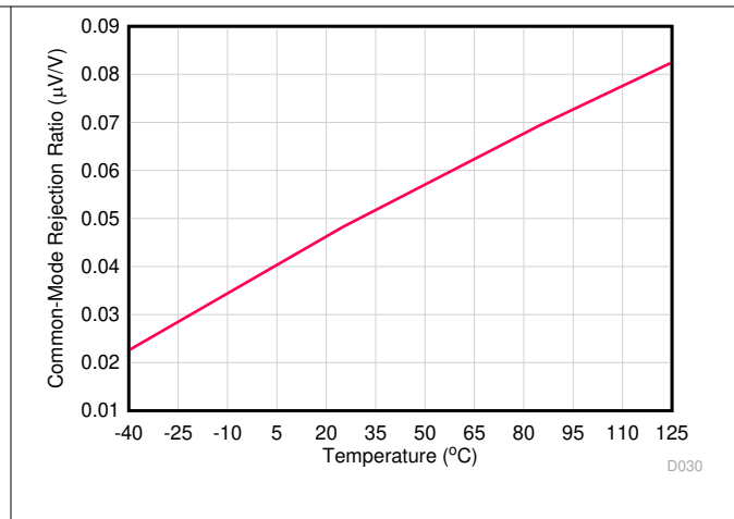
图 6-8. Common Mode Rejection Ratio vs Temperature
