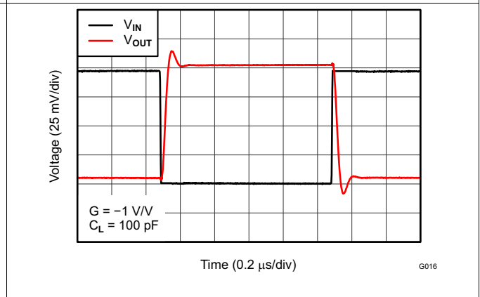
图 16. Small-Signal Step Response (100 mV)
