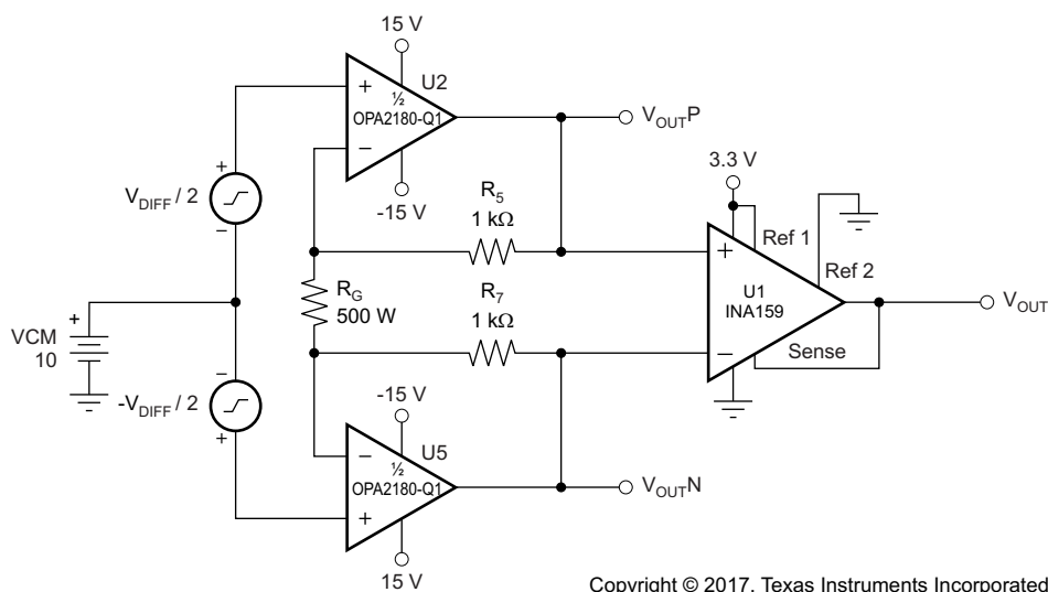
图 33. Discrete INA + Attenuation for ADC With a 3.3-V Supply
