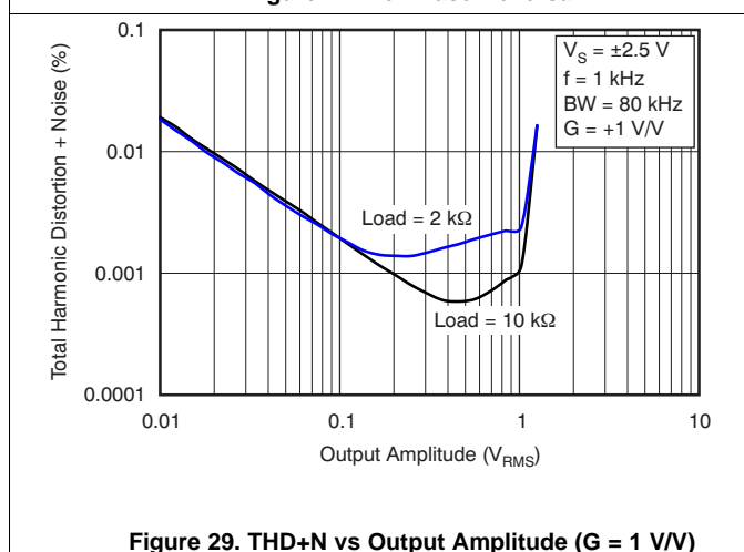
Figure 29. THD+N vs Output Amplitude ( G = 1\text{ V/V} )
