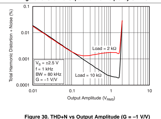
Figure 30. THD+N vs Output Amplitude ( G = -1\text{ V/V} )
