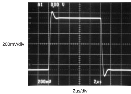
SMALL SIGNAL RESPONSE G = 3 , C_L = 1\text{nF}
