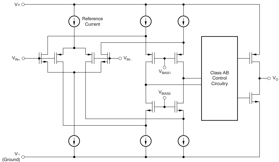
Figure 33. Simplified Schematic
