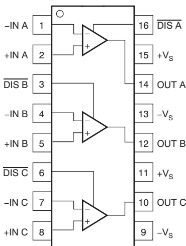
D AND DBQ PACKAGES SO-16 AND SSOP-16 (TOP VIEW)
