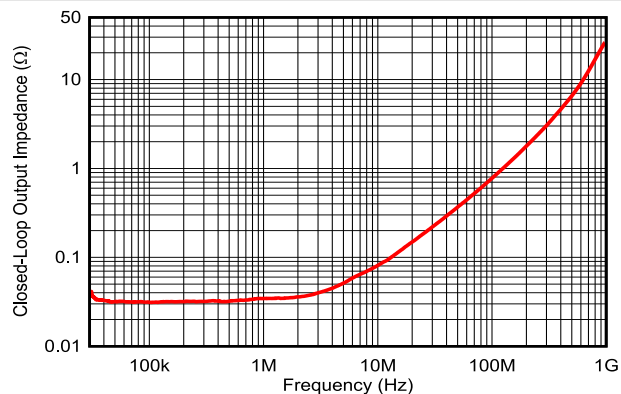
图 6-6. Closed-Loop Output Impedance vs Frequency
