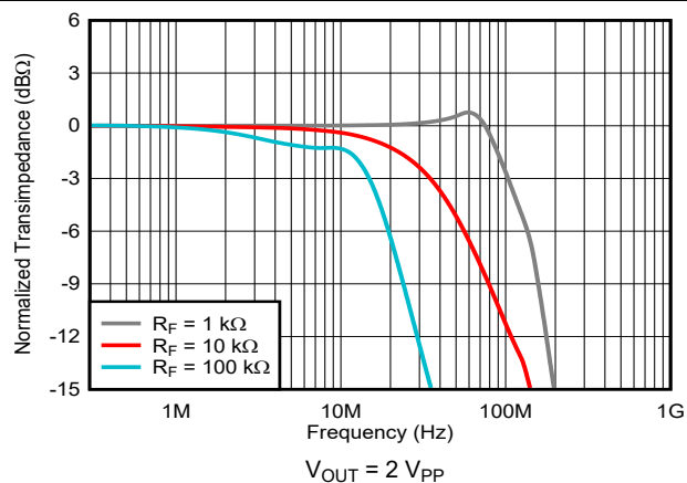
图 6-4. Large-Signal Frequency Response vs Gain
