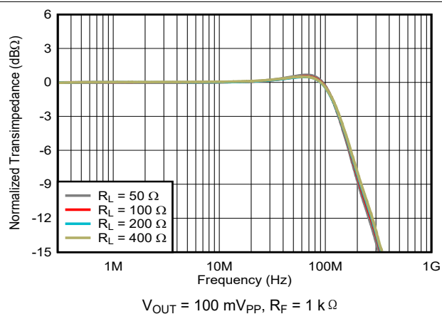
图 6-2. Small-Signal Frequency Response vs Output Load
