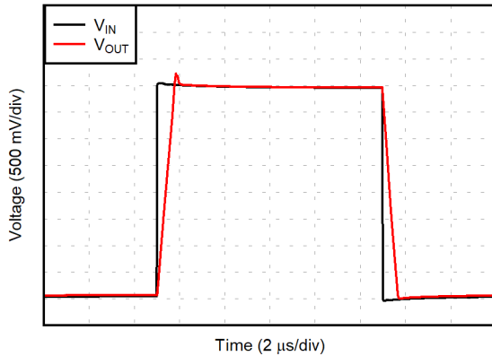
Time (2 \mu\text{s}/\text{div} ) G = 1
