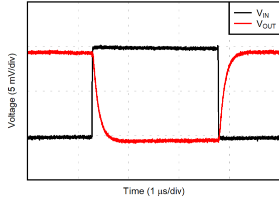
Time (1 \mu\text{s}/\text{div} ) G = -1
