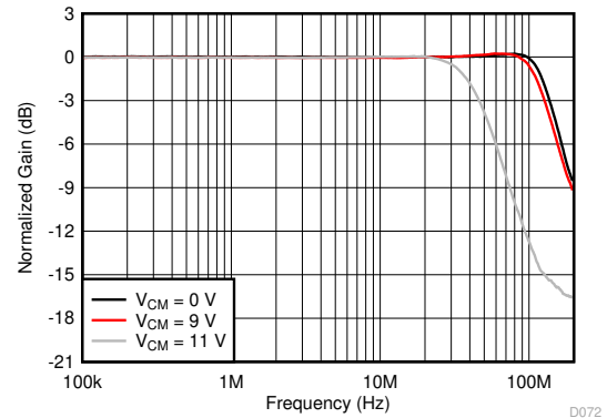
图 6-19. Small-Signal Frequency Response vs Output Common-Mode Voltage
