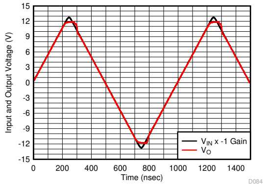
图 6-30. Output Overdrive Recovery
