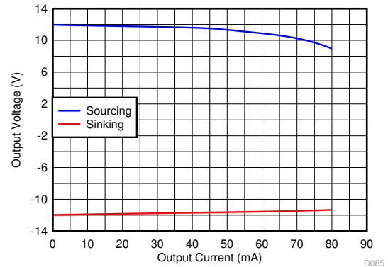
图 6-31. Output Voltage Range vs Load Current
