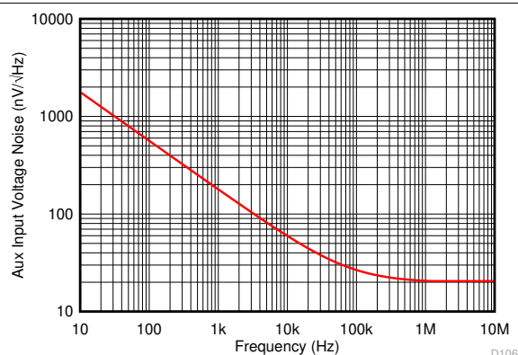
图 6-48. Auxiliary Input Stage Voltage Noise Density vs Frequency
