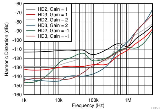
图 6-8. Harmonic Distortion vs Frequency
