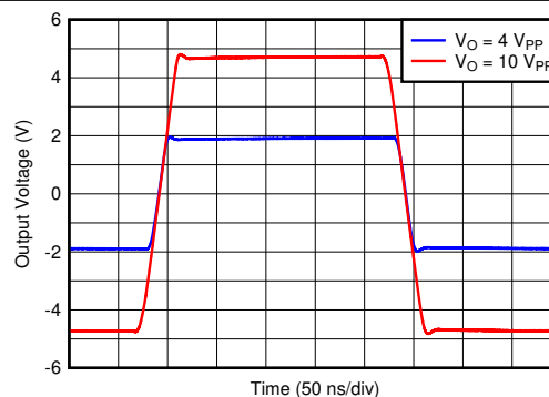
图 6-25. Large-Signal Transient Response
