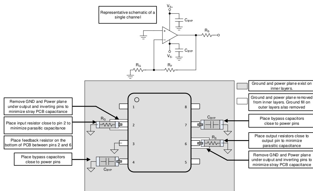
图 8-19. Layout Recommendation
