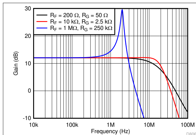
图 8-8. Closed-Loop Gain vs. Frequency for Circuit of 图 8-5
