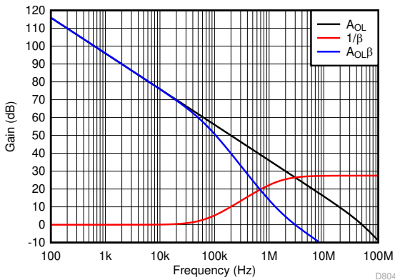
图 8-13. Loop-Gain Magnitude vs Frequency for the Transimpedance Amplifier Circuit of 图 8-12
