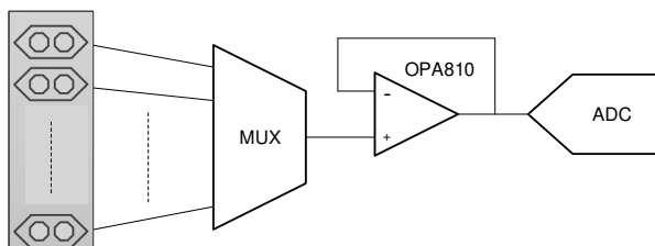
图 8-17. Multichannel Sensor Interface Using a Single Higher GBWP Amplifier
