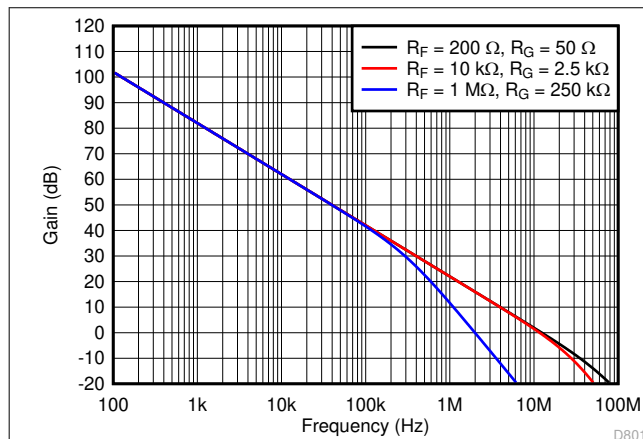
图 8-6. Loop-Gain vs Frequency for Circuit of 图 8-5
