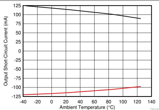
图 6-40. Output Short-Circuit Current vs Ambient Temperature
