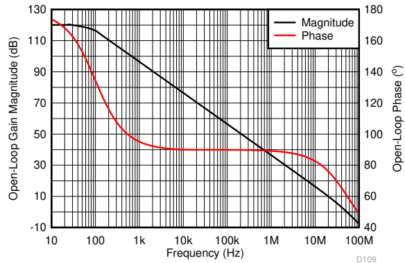
图 6-42. Open-Loop Gain and Phase vs Frequency
