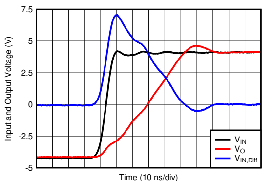
图 8-18. Large-Signal Transient Response Using the OPA810
