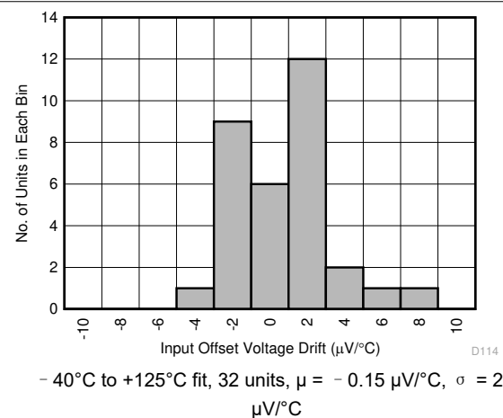
图 6-59. Input Offset Voltage Drift Distribution
