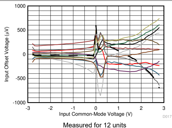
图 6-41. Input Offset Voltage vs Input Common-Mode Voltage
