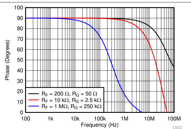
图 8-7. Loop-Gain Phase vs Frequency for Circuit of 图 8-5
