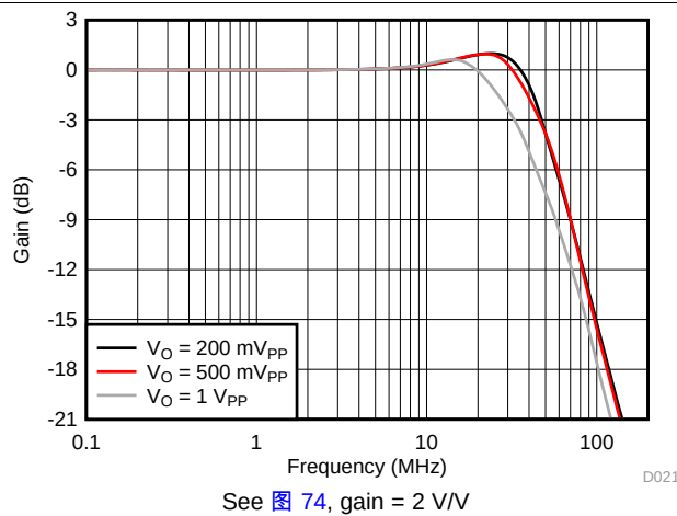
图 21. Noninverting Large-Signal Bandwidth vs V_{OPP}
