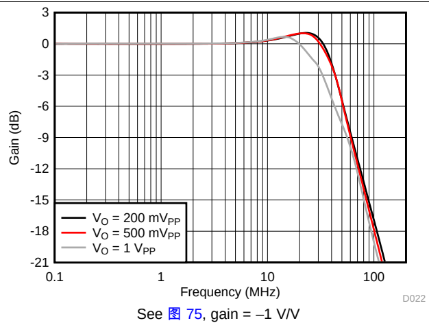
图 22. Inverting Large-Signal Bandwidth vs V_{OPP}
