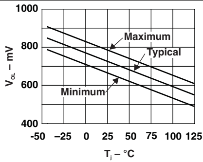
Figure 1. V_{OL} at Sx vs Junction Temperature, I_{OL} = 0.2 mA
