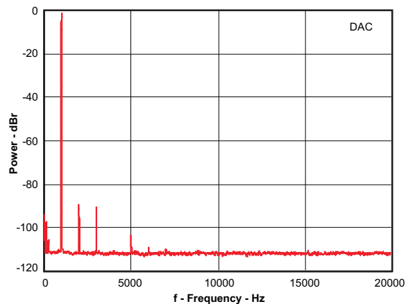
Figure 14. Playback to Headphone FFT at -1dBr vs Frequency
