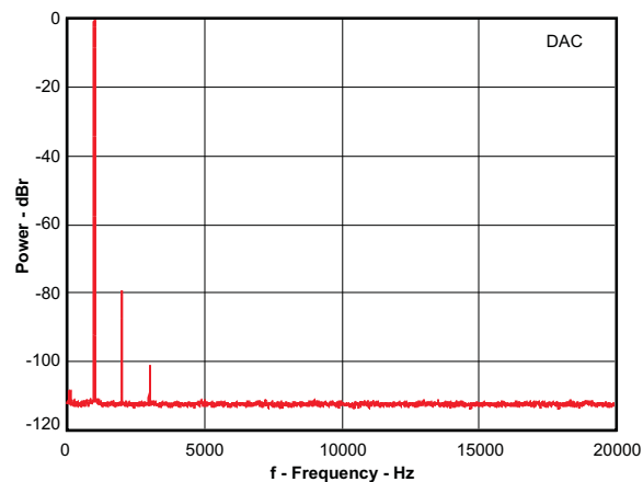
Figure 15. DAC Playback to Line-out FFT at -1dBr vs Frequency
