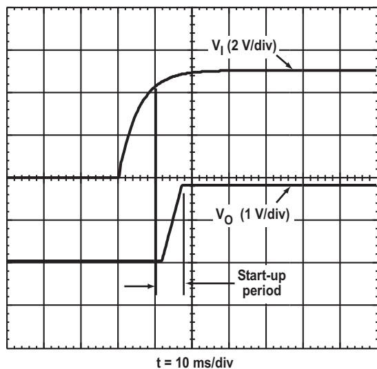
Figure 14. PTV05010W Start-Up
