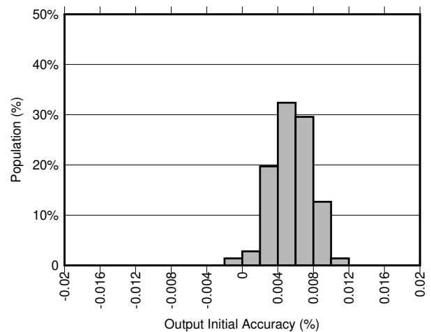
图 7-6. Accuracy Distribution (REF7025QFKHR)
