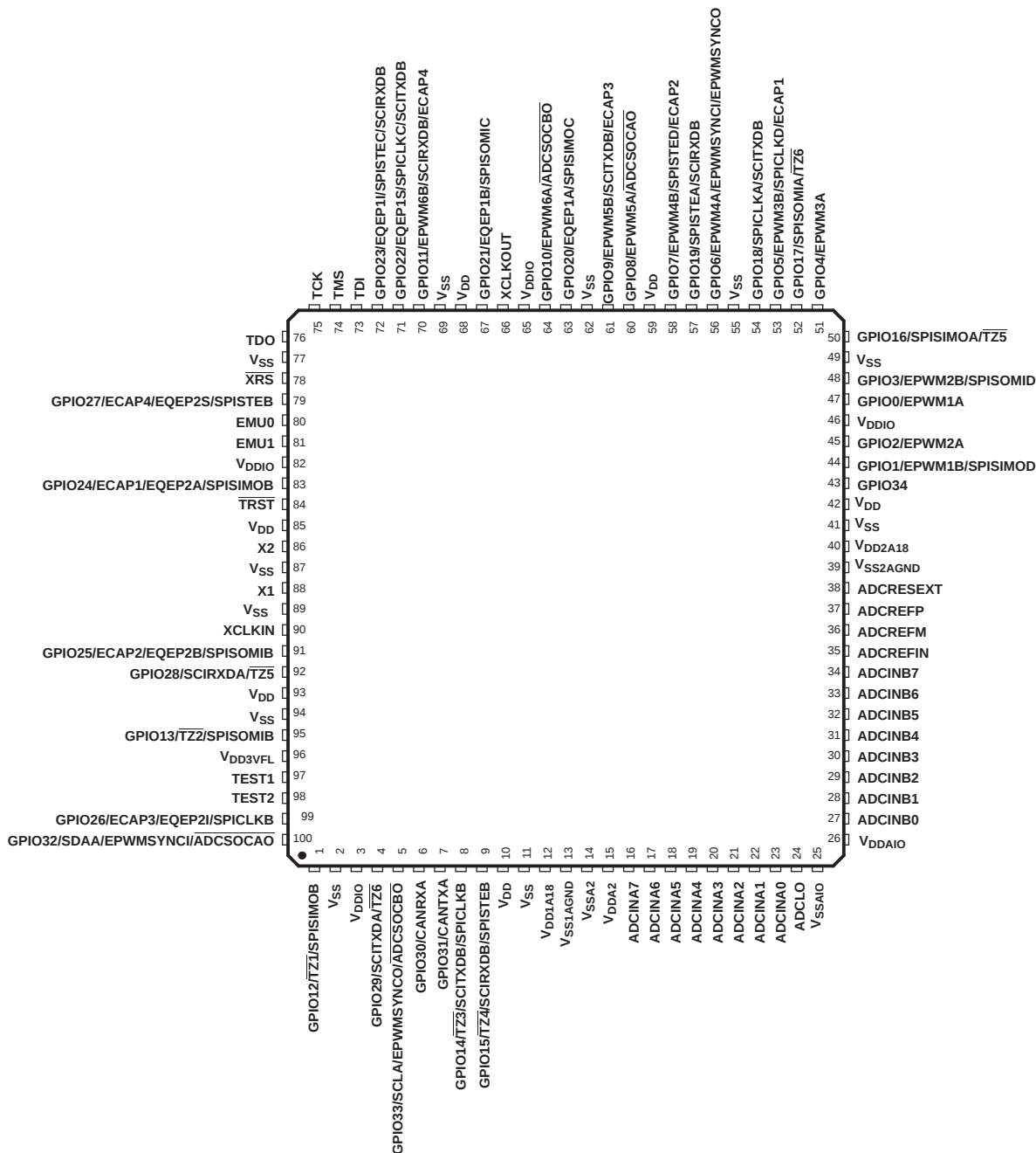
Figure 2-2. F2806 100-Pin PZ LQFP (Top View)
