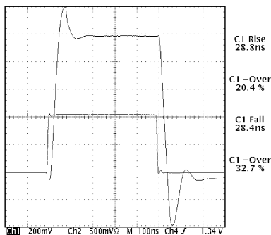
Figure 57. R_C = 330\Omega and C = 10\text{ nF} , Gain = +1
