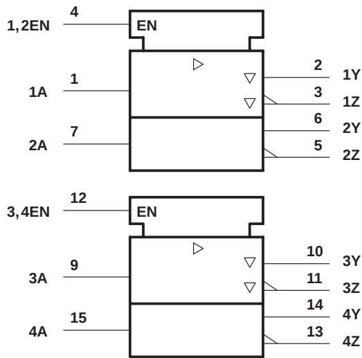
logic symbol†
