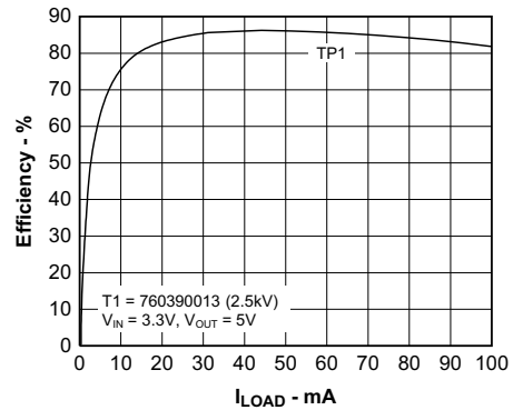
图 5-6. Efficiency vs Load Current
