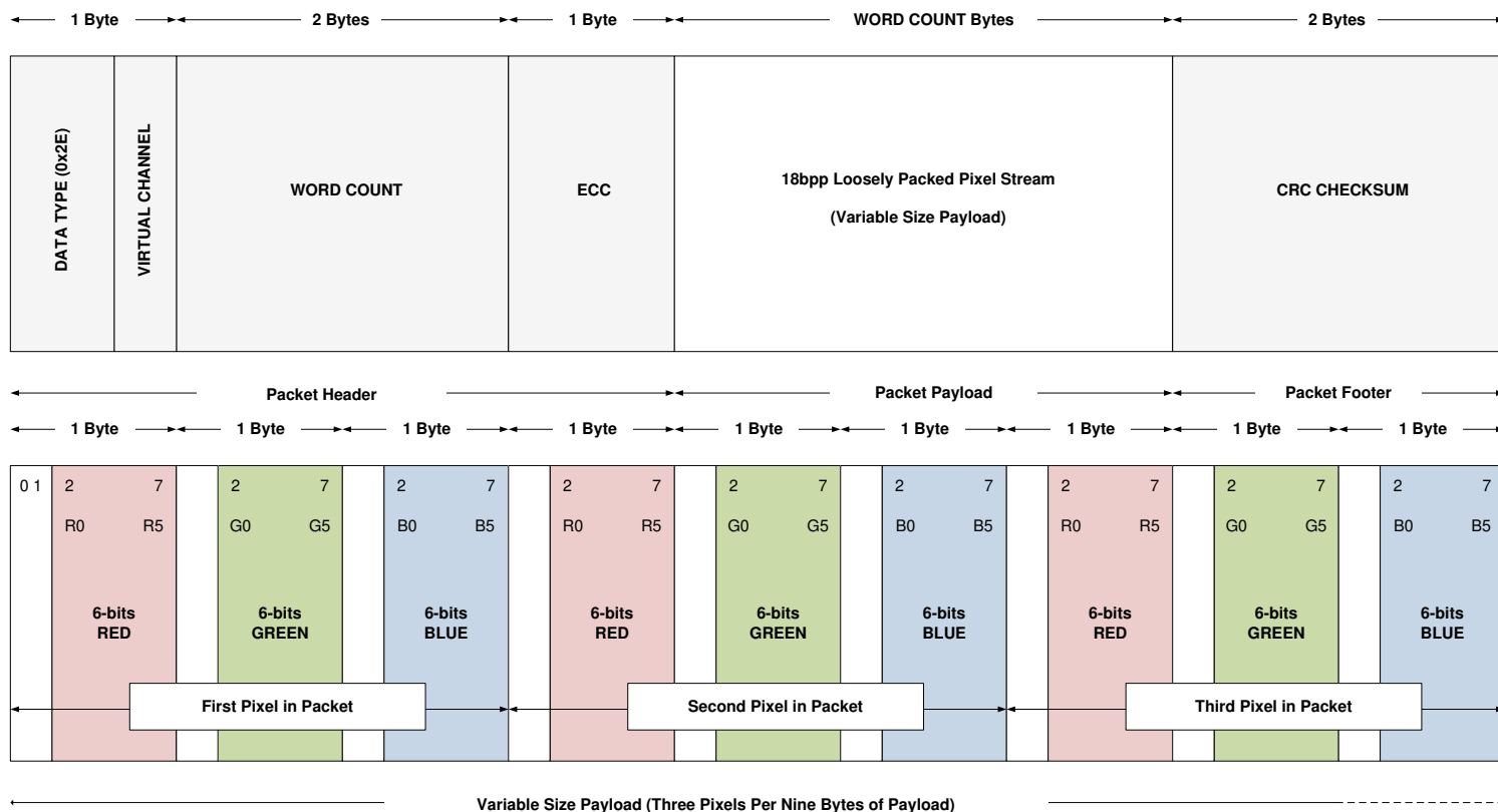
图 8-7. 18 bpp (Loosely Packed) DSI Packet Structure
