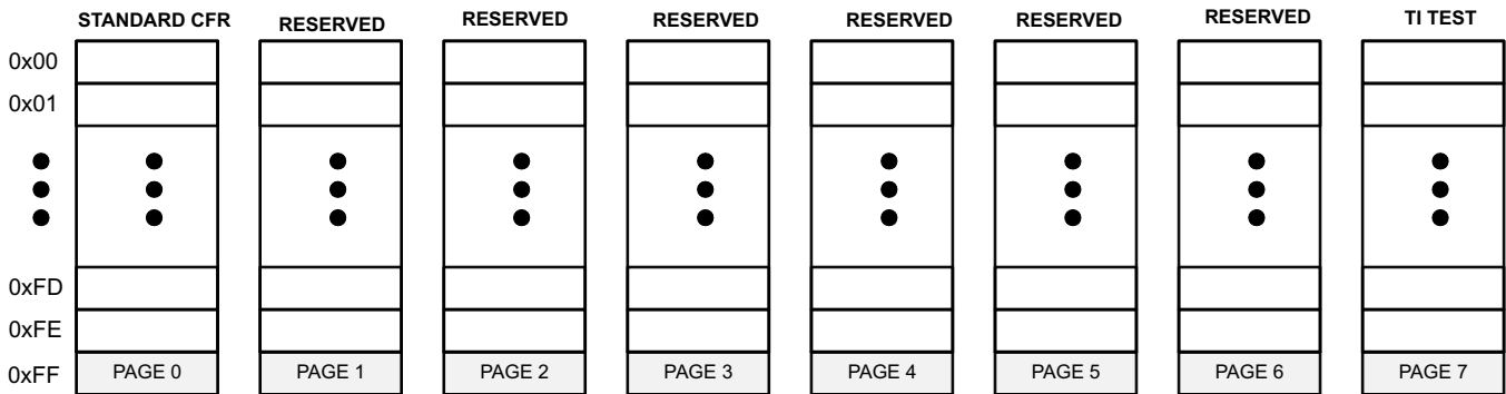
Figure 19. Register Map
