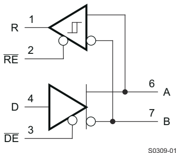
图 9-3. SN65HVD1708E Transceiver for J1708 Applications
