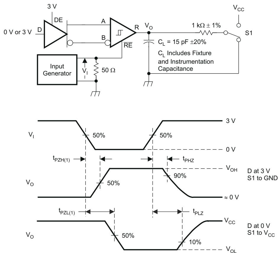
图 8-7. Measurement of Receiver Enable/Disable Times With Driver Enabled
