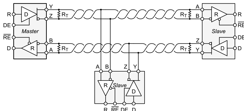
图 10-2. Typical RS-485 Network With Full-duplex Transceivers
