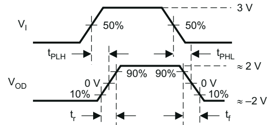
图 8-3. Measurement of Driver Differential Output Rise and Fall Times and Propagation Delays
