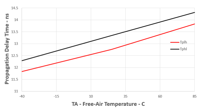
图 5-4. Propagation Delay Time vs Free-air Temperature
