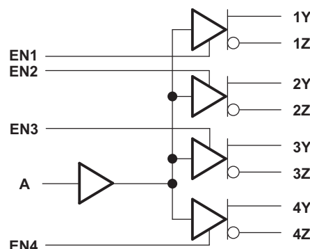
SN65LVDS105 Logic Diagram (Positive Logic)
