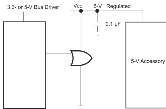
图 9-1. Typical Application Diagram for a Single Gate
