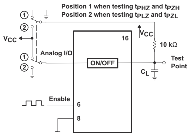
图 6-10. Propagation-Delay Test Setup, Enable to Analog Out
