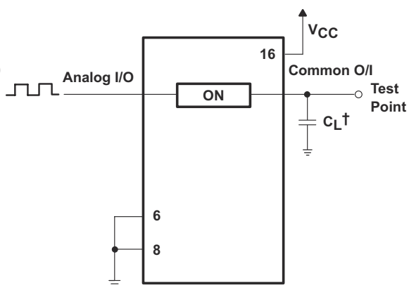
图 6-8. Propagation-Delay Test Setup, Analog In to Analog Out
