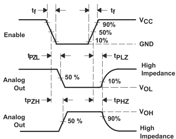
图 6-9. Propagation Delays, Enable to Analog Out
