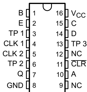
Pin Functions, SN74LS292
