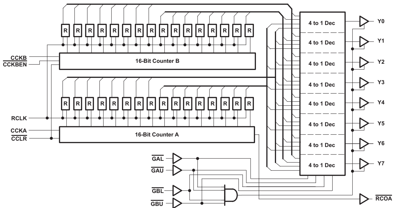
Simplified Schematic
