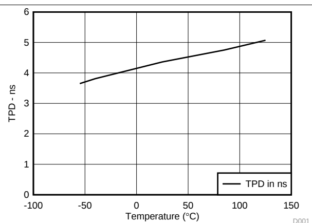
Figure 2. SN74LVC373A LE to Q TPD Across Temperature at 3.3-V V_{CC}
