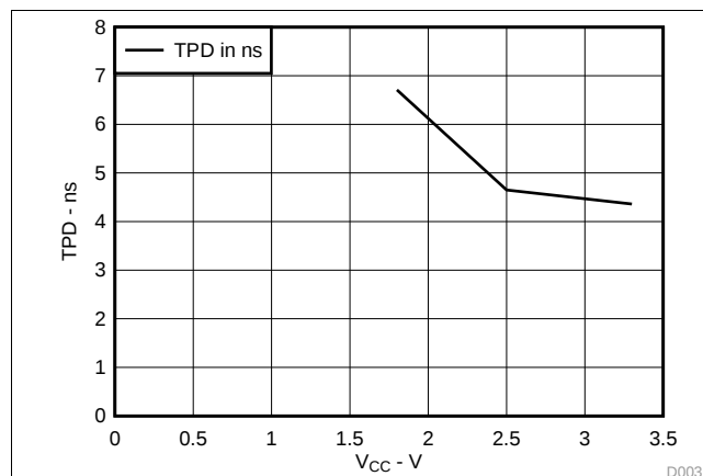
Figure 1. SN74LVC373A LE to Q TDP V_{CC} vs TPD at 25^\circ\text{C}
