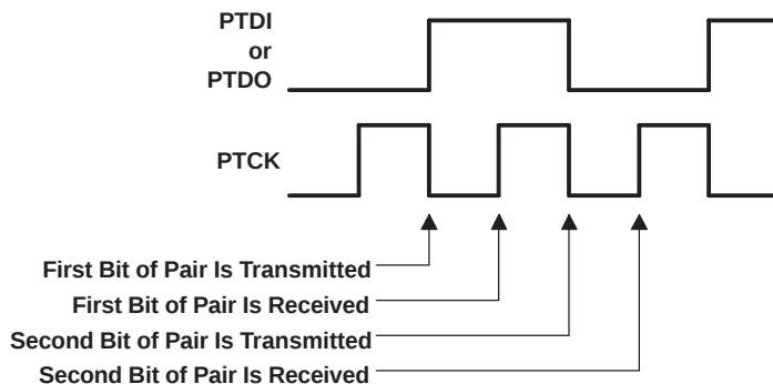
Figure 2. Bit-Pair Timing (Data Zero Shown)
