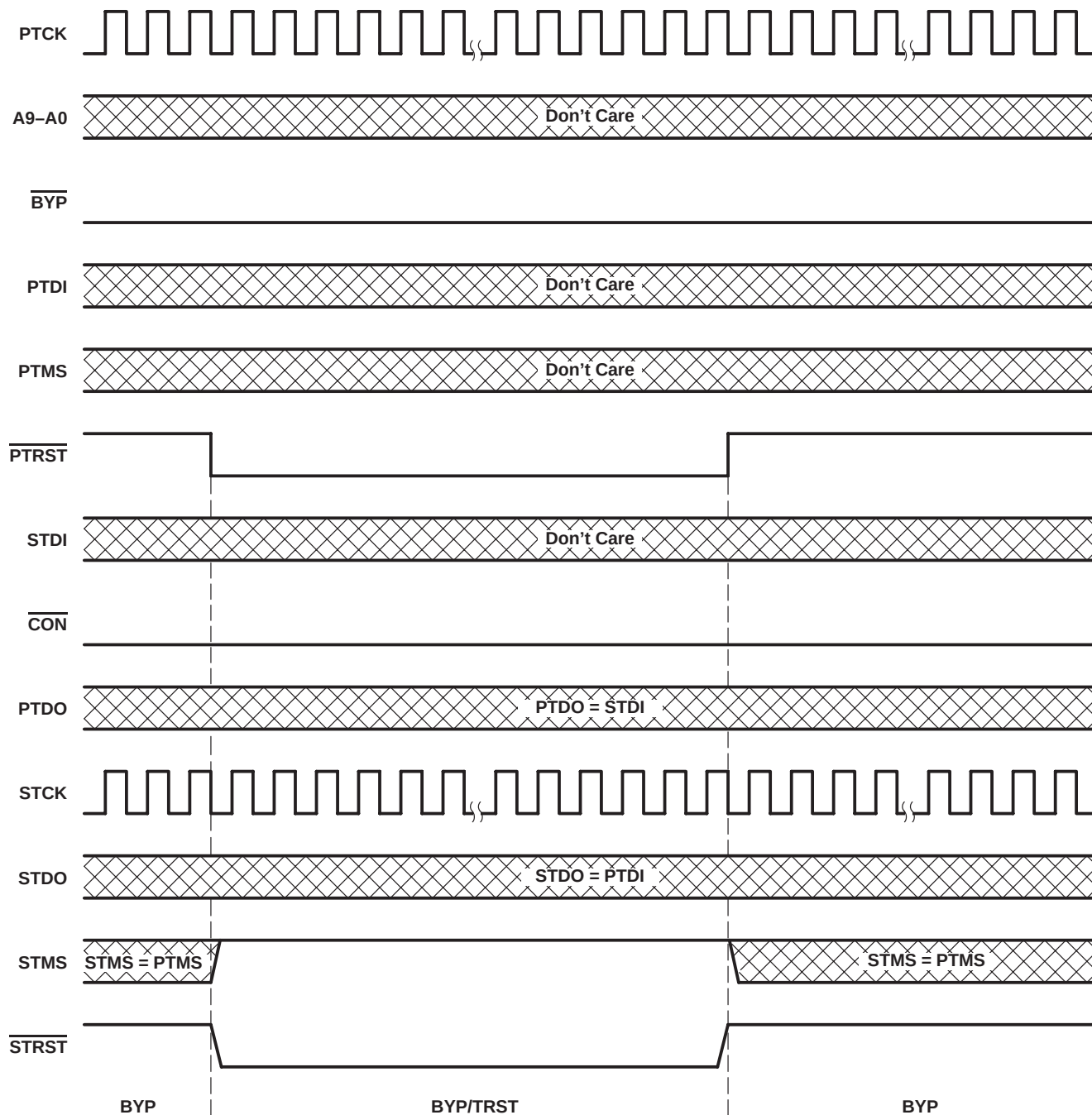
Figure 23. Asynchronous Reset Timing, \overline{BYP} = L
