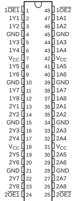
SN54LVTH162541 . . . WD PACKAGE SN74LVTH162541 . . . DGG OR DL PACKAGE (TOP VIEW)
