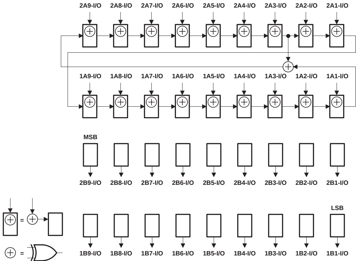
Figure 12. 18-Bit PSA/COUNT Configuration (10EAB = 20EAB = 1, 10EBA = 20EBA = 1)
