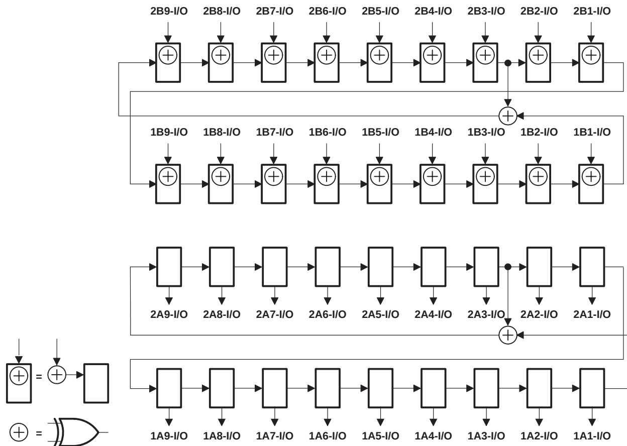
Figure 11. 18-Bit PSA/PRPG Configuration (1OEAB = 2OEAB = 0, \overline{1OEBA} = \overline{2OEBA} = 0 )
