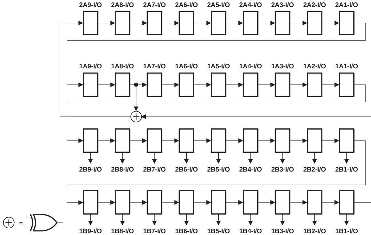
Figure 6. 36-Bit PRPG Configuration (1OEAB = 2OEAB = 1, \overline{1OEBA} = \overline{2OEBA} = 1 )
