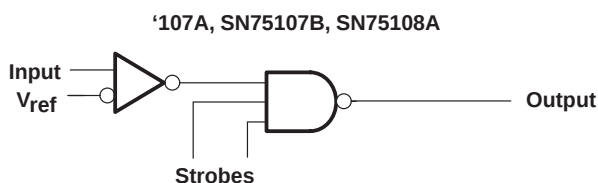
Figure 13. Single-Ended Operation
