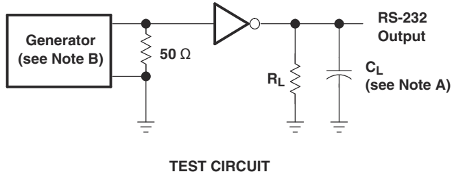
图 7-1. Driver Slew Rate
