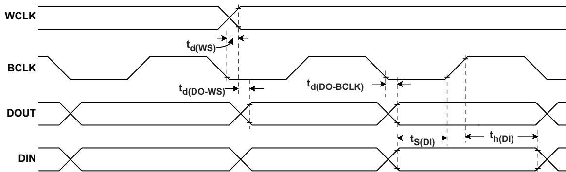
图 3. I²S/LJF/RJF Timing in Master Mode
