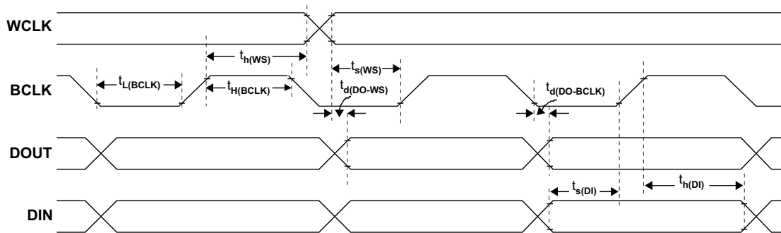
图 4. I²S/LJF/RJF Timing in Slave Mode
