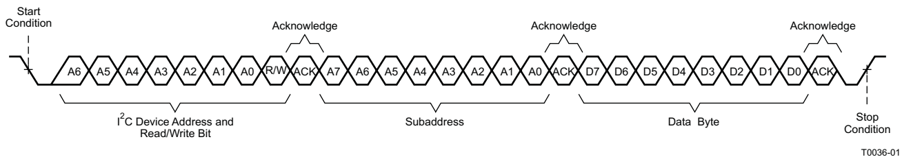
Figure 16. Random-Write Transfer
