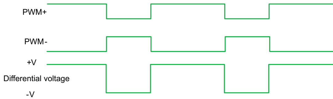
Figure 20. AD Modulation
