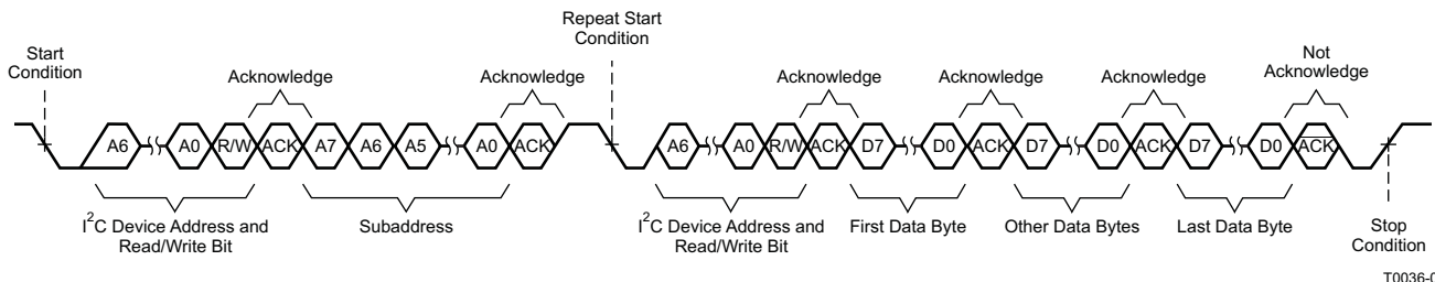
Figure 30. Multiple Byte Read Transfer
