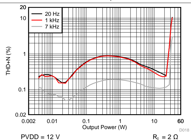
图 22. THD+N vs Output Power - PBTL
