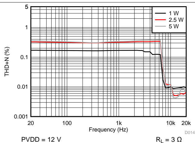
图 18. THD+N vs Frequency - PBTL
