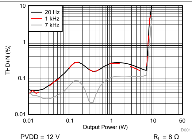
图 10. THD+N vs Output Power - BTL
