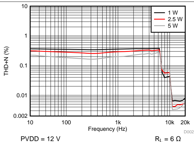
图 8. THD+N vs Frequency - BTL
