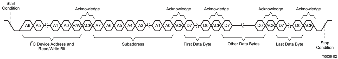
图 52. Multiple-Byte Write Transfer
