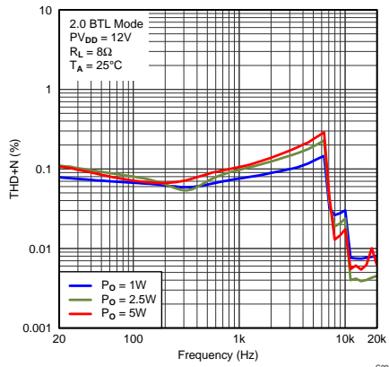
图 7. THD+N vs Frequency
