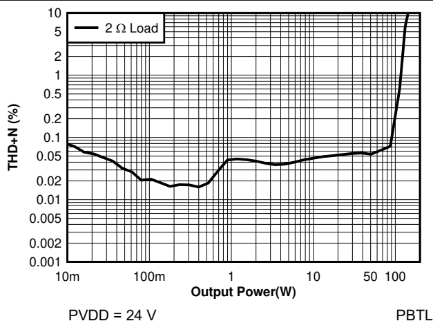
图 7-29. THD+N vs Power - PBTL - 24 V
