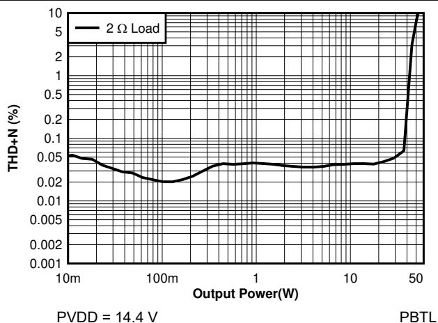
图 7-28. THD+N vs Power - PBTL - 14.4V
