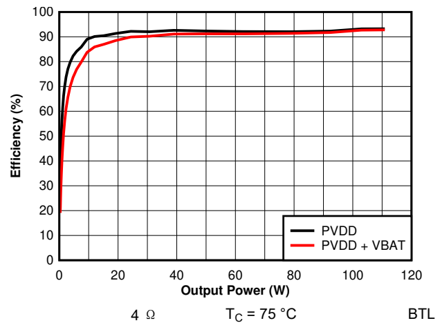
图 7-22. Efficiency vs Output Power - 4 \Omega - 384 kHz
