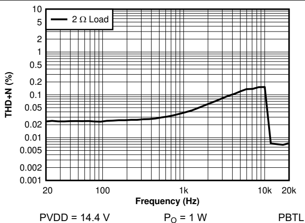
图 7-30. THD+N vs Frequency - PBTL - 14.4 V
