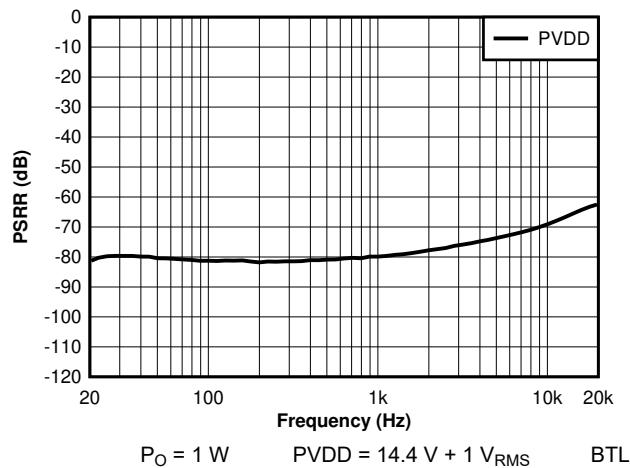
图 7-16. PSRR vs Frequency - PVDD Only
