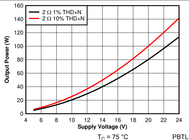
图 7-32. Output Power vs Supply Voltage - PBTL
