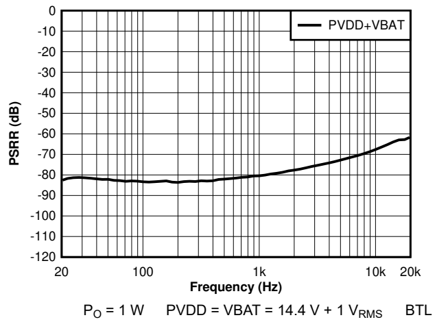
图 7-18. PSRR vs Frequency - PVDD + VBAT
