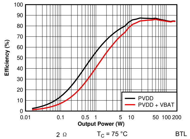
图 7-26. Efficiency vs Output Power - 2 \Omega - 384 kHz (Zoomed)
