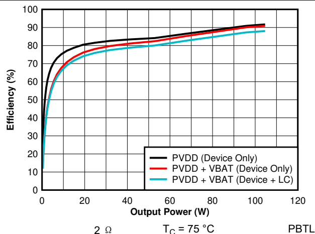
图 7-33. Efficiency vs Output Power - PBTL - 2 \Omega
