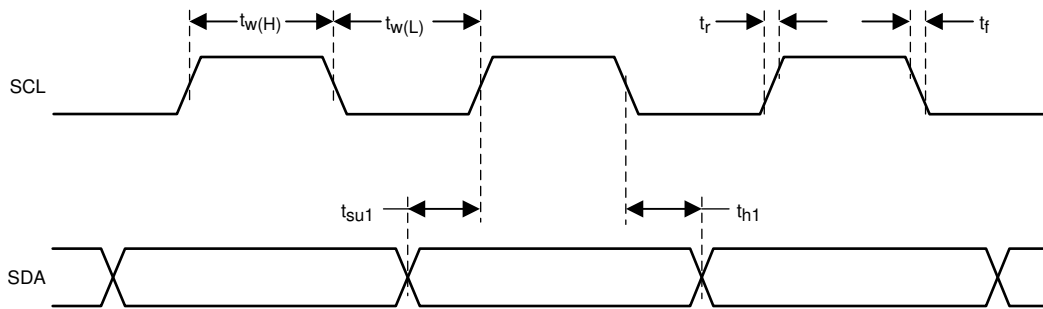
图 9-9. SCL and SDA Timing
