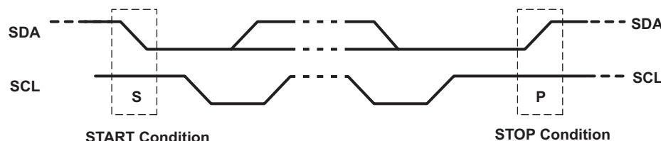
Figure 9. Definition of Start and Stop Conditions
